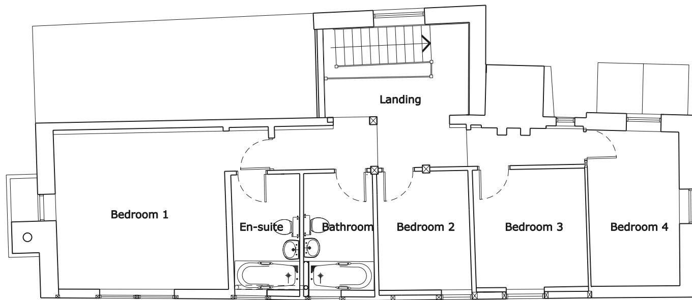
LITTLE CANWOOD HOUSE - FIRST FLOOR PLAN
